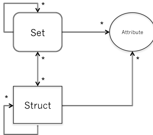
Figure 5.3: The metalayer
