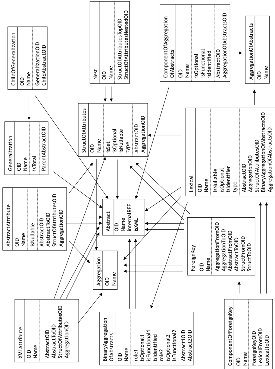
Figure 1.3: The supermodel
