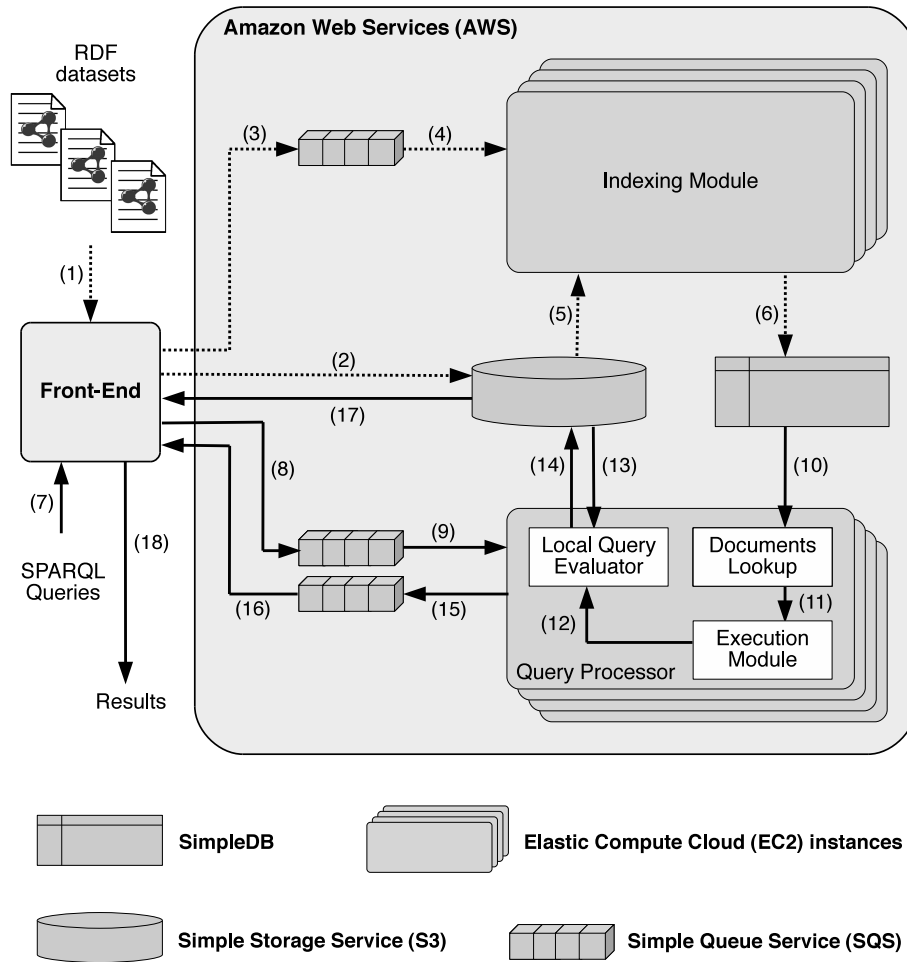
Figure 6.3: Proposed architecture.
