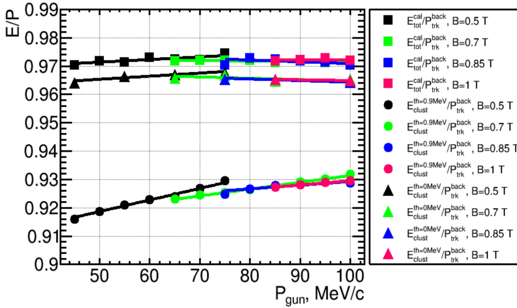
Figure 7.34: E/P distribution for three different clustering threshold as a function of the generated momentum value.
