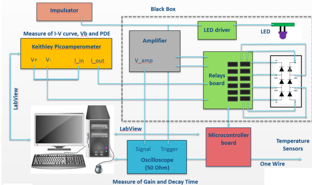
Figure 5.3: Scheme of the experimental setup used for the pre-production SiPMs tests.
