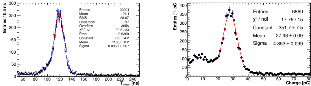
Figure 4.11: Left: Time distribution mean value, fitted with a gaussian function to evaluate the mean value and the \sigma of the distribution. Events are selected only if their peak time is around \pm 3\sigma of the mean value. Right: Charge distribution of the crystal under test after the timing selection and the TAG charge cuts.
