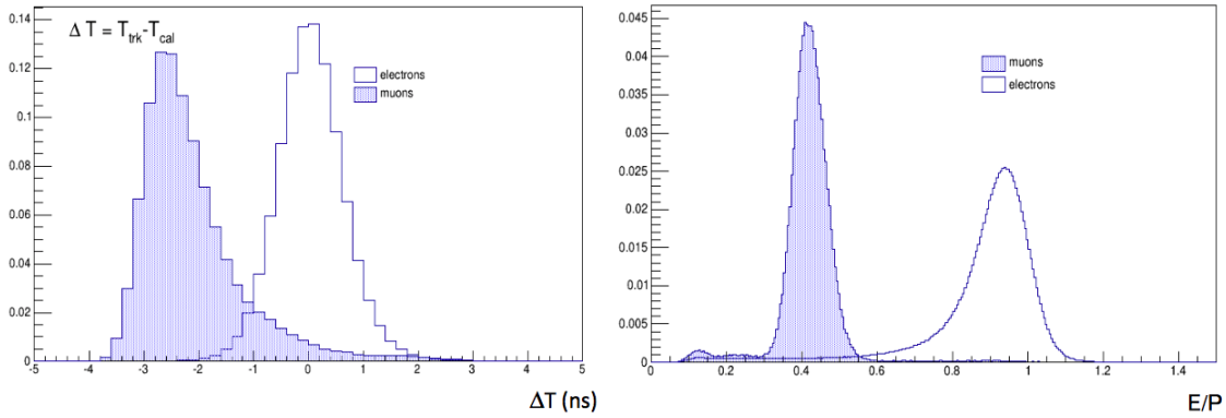
Figure 3.23: Distributions of time difference, \Delta t , between the track and the cluster (left) and E/P (right) for 105 MeV/c electrons and muons [1].
