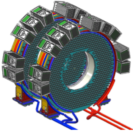
Figure 3.1: Calorimeter design.
