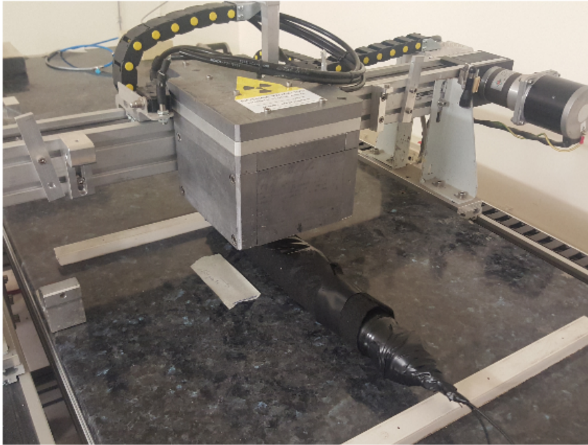
Figure 4.17: Experimental apparatus for RIN measurements: a motorized cart transport a strong ^{137}\text{Cs} source over the CUT.
