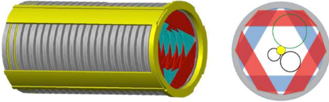
Figure 2.10: Left: The Mu2e straw tube tracker. The straws are oriented transverse to the solenoid axis. Right: cross sectional view of the Mu2e tracker station with the trajectories of a 105 MeV CE (top) and a 53 MeV Michel electron (lower right) superimposed. The disk in the center is the stopping target. Electrons with energies smaller than 53 MeV (lower left) miss the tracker entirely.
