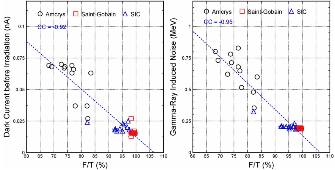
Figure 4.20: Dark current before the irradiation (left) and \gamma -RIN (right) measurements as a function of the F/T ratio.
