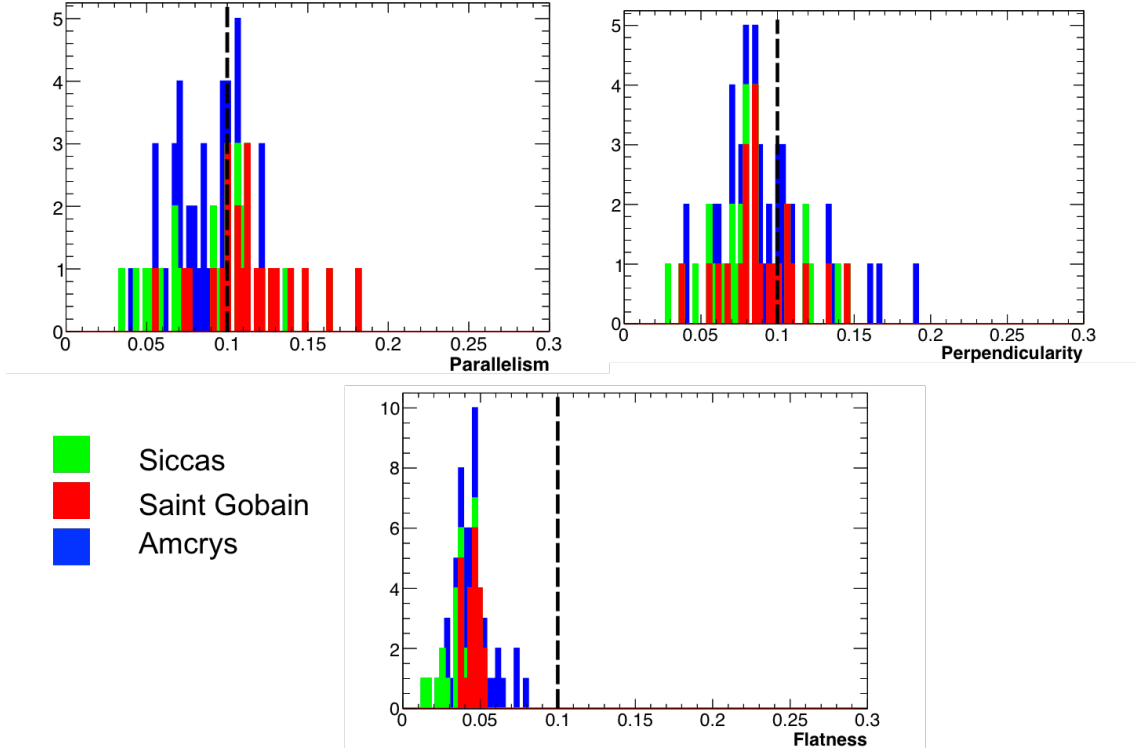
Figure 4.4: Stack distribution of the shape tolerances for the 72 pre-production crystals. Black dashed lines shows the limits imposed by the mechanical requirements.
