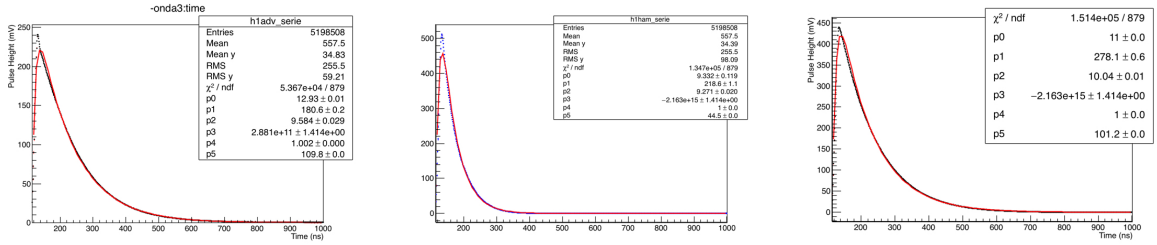
Figure 5.15: Average waveform for a a single cell of the AdvanSiD (left), Hamamatsu (middle) and SensL (right) SiPM.
