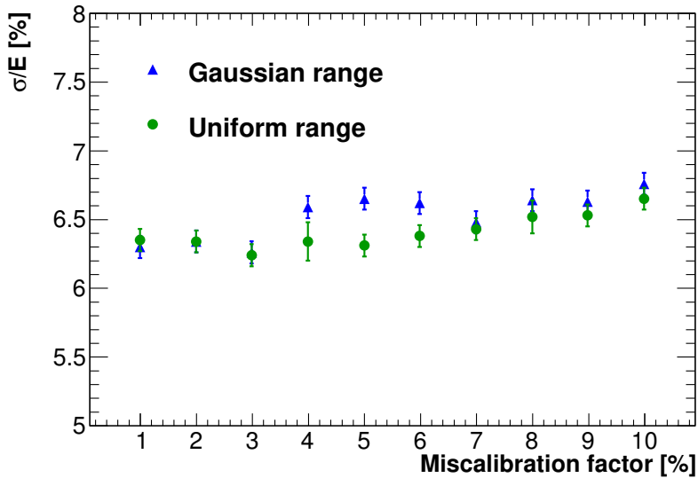
Figure 7.1: Energy resolution as a function of the miscalibration coefficient inserted in the MC simulation.
