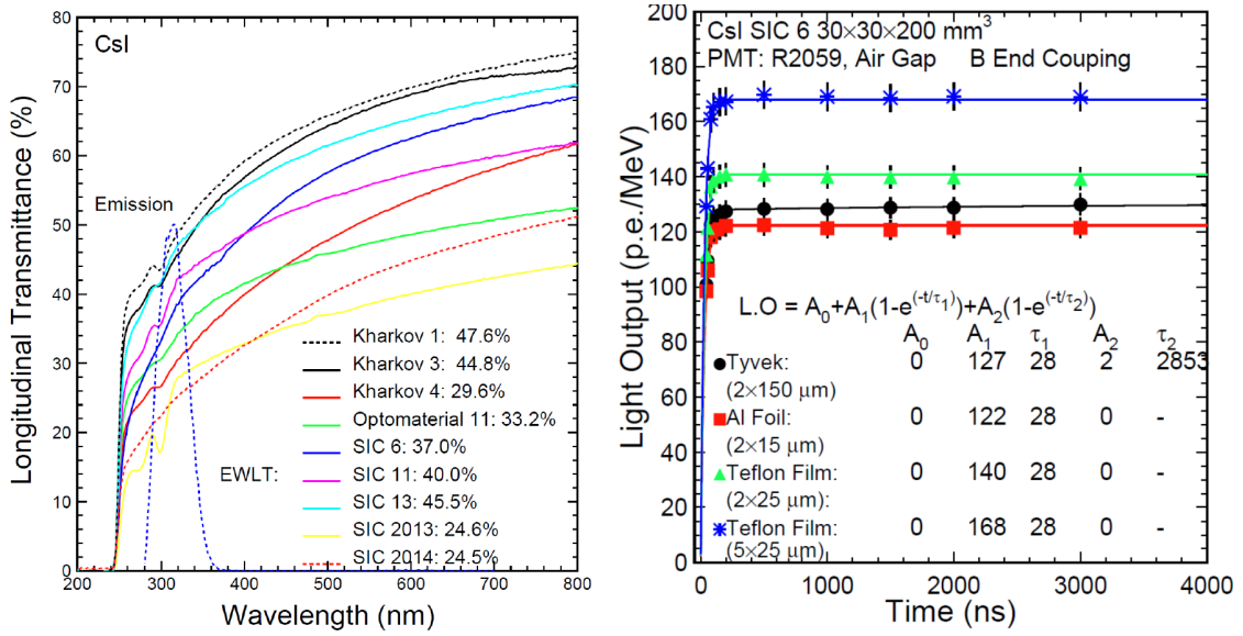
Figure 4.5: CsI EWLTL (left) and light output (right).
