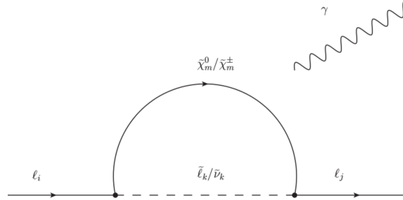
Figure 1.5: Supersymmetric contribution to l_i \rightarrow l_j\gamma , l_i - N \rightarrow l_j N . It is understood that the photon attaches to the fermion or the scalar in the loop, depending on which field is charged.
