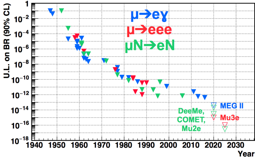
Figure 1.9: Limits on the branching ratio of the CLFV processes involving muon evaluated experimentally during last years and in future experiments (empty triangles).
